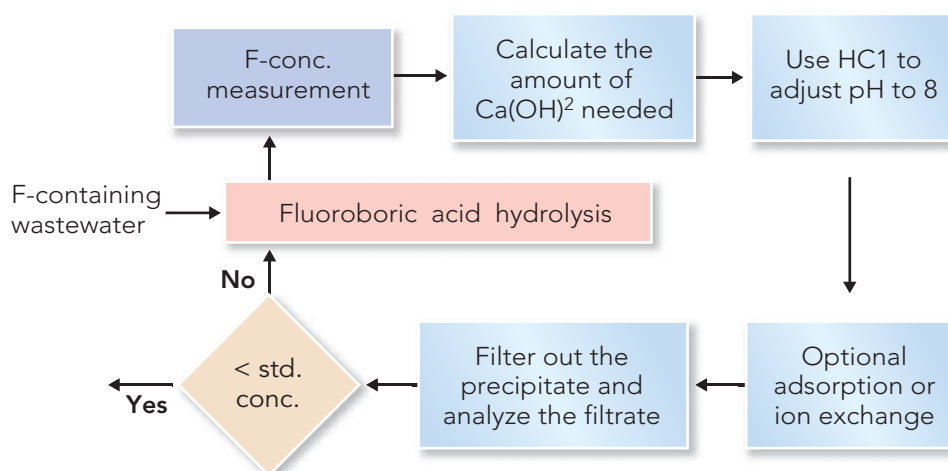
▲ Process for treating F-containing wastewater
