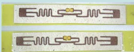
▲ Rfid Antenna with Plating Nickel-gold
