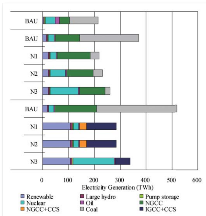
▲ The Allocation of Electricity Generation for the BAU and Reduction Scenarios
