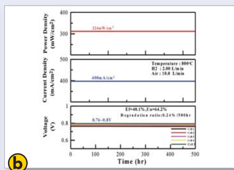
▲ (a) The Performance Curves of a 40-cell kW-level Stack; (b) Durability Testing Curves of a 5-cell Stack.
