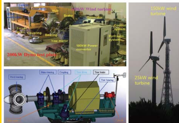
▲ Dynamic Testing Systems for 25 kW and 150 kW Wind Turbine
