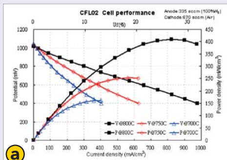
▲ The Performance Curves of the (a) Anode Supported Cell (ASC); (b) Metal Supported Cell (MSC).
