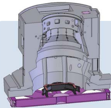
▲ Profile of Potential Clearance Region
