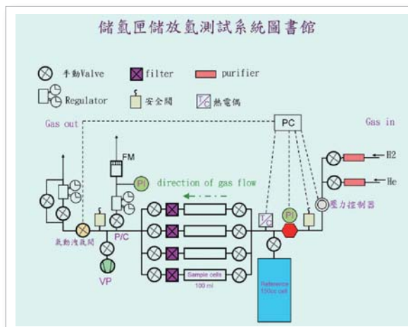
▲ Schematic Diagram of the Hydrogen Desorption System for the Cartridge with Large Amount of Pt/AC Samples
