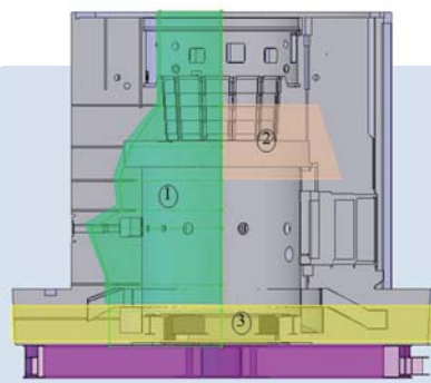
▲ Activated Region of Biological Shielding
