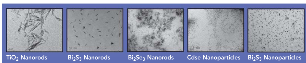
▲ The TEM Images of \text{TiO}_2 , CdSe, \text{Bi}_2\text{S}_3 and \text{Bi}_2\text{Se}_3 Quantum Dots.
