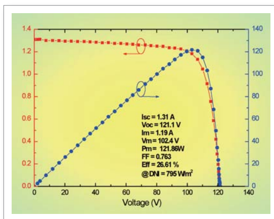
▲ I-V & P-V Curve of Solar Module under 900 Geometric Concentration Ratio
