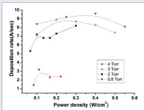
▲ The Variation of Growth rate as a Function of Power Density at Different Chamber Pressures in a VHF PECVD System
