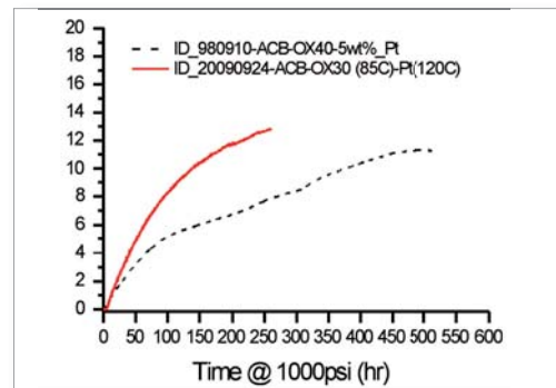
▲ Pt/AC Samples with Different Pt Impregnation Processes Showing Different Hydrogen Uptake Rates but nearly the Same Storage Capacities
