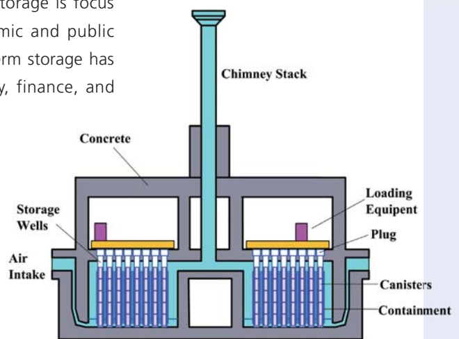
▲ Concept of Storage Building.
