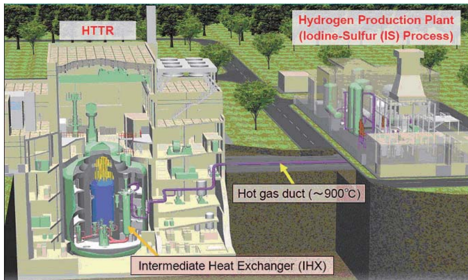
▲ Illustration of Hydrogen Generation Facility for HTTR
