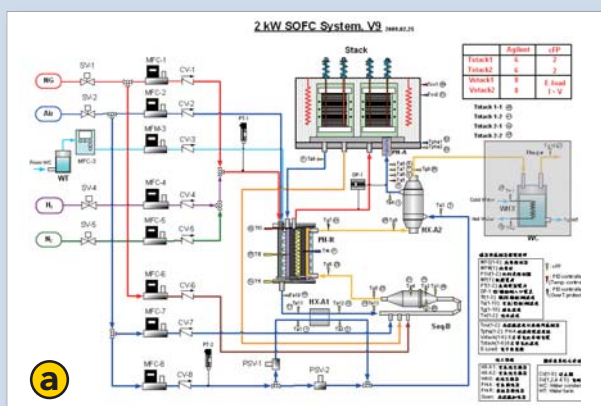
▲ The First Generation of the 2 kW Power Generating System: (a) Piping and Instrument Diagram; (b) Heating-up Testing Curves.
