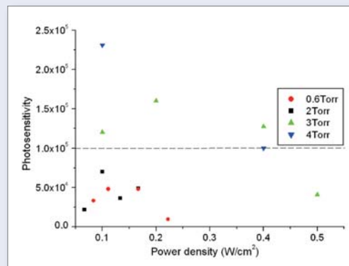
▲ The Photosensitivity of I-layer of amorphous Silicon Films as a Function of Power Density at Different Chamber Pressures Deposited in a VHF PECVD System
