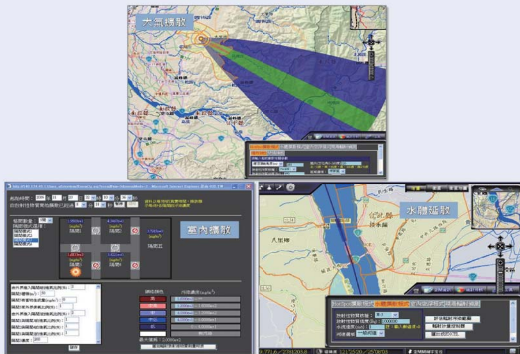
▲ The Short-lived Radionuclide-dispersion Models of Rdd: Atmospheric Dispersion, Dispersion in Complex Building Environments and Terrestrial Surface Water Bodies
