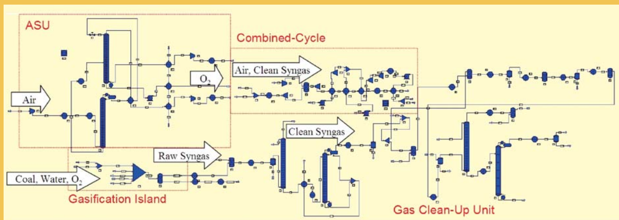
▲ IGCC Simulation Model
