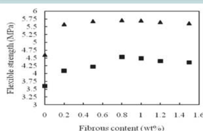
▲ Flexural Strength of Fibrous Reinforcement Concrete; ■: 7days; ▲: 28days
