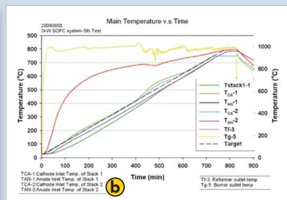
▲ The First Generation of the 2 kW Power Generating System: (a) Piping and Instrument Diagram; (b) Heating-up Testing Curves.
