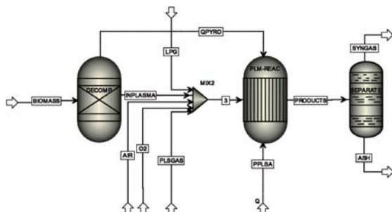
▲ Process Simulation for Plasma Gasification System.
