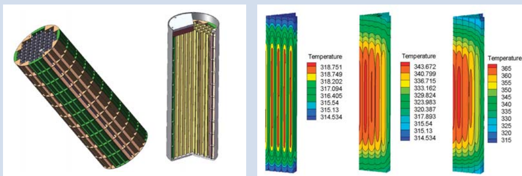
▲ 3d Diagram of the Transportable Steel Canister (Tsc) and Tube-type Basket.
