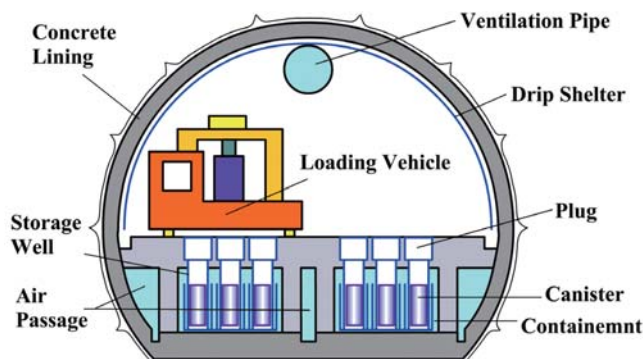
▲ Concept of Storage Cavern.
