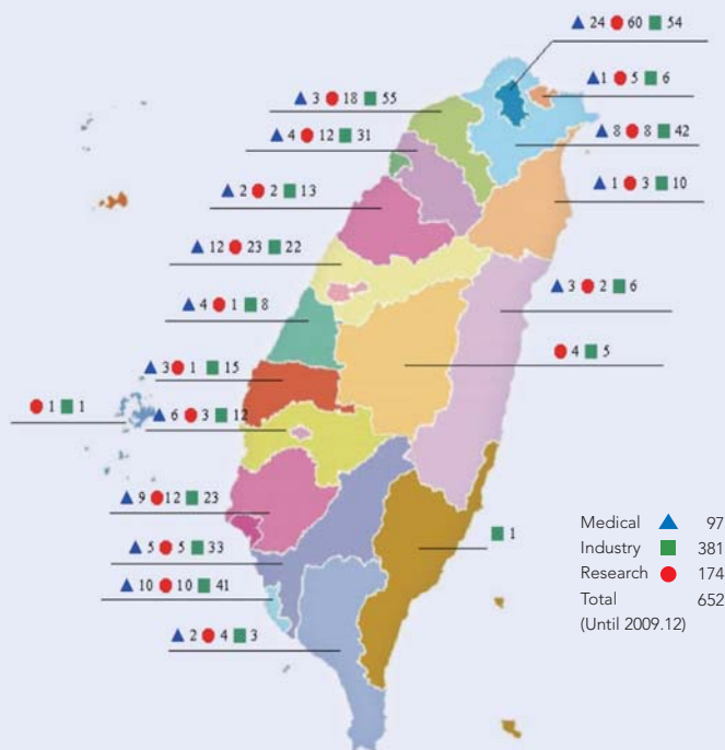
▲ Distributions of the Low Level Radioactive Wastes Accepted by INER and Generated from Small User Facilities
