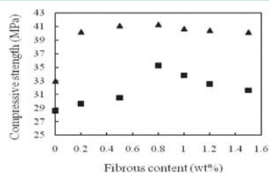
▲ Compressive Strength of Fibrous Reinforcement Concrete; ■: 7days; ▲: 28days
