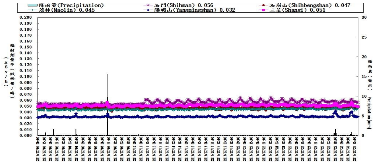
Hourly average dose rates around NPPI in Taiwan (July, 2017)
