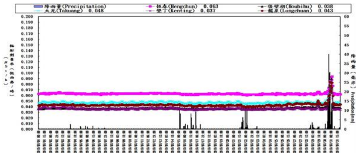
核三廠輻安預警自動監測時平均劑量率(中華民國一百零六年七月) Hourly average dose rates around NPP3 in Taiwan (July, 2017)
