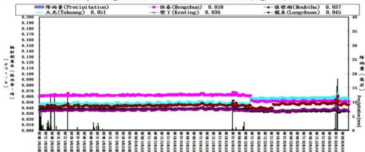
核三廠輻安預警自動監測時平均劑量率(中華民國一百零六年九月) Hourly average dose rates around NPP3 in Taiwan (Sep, 2017)
