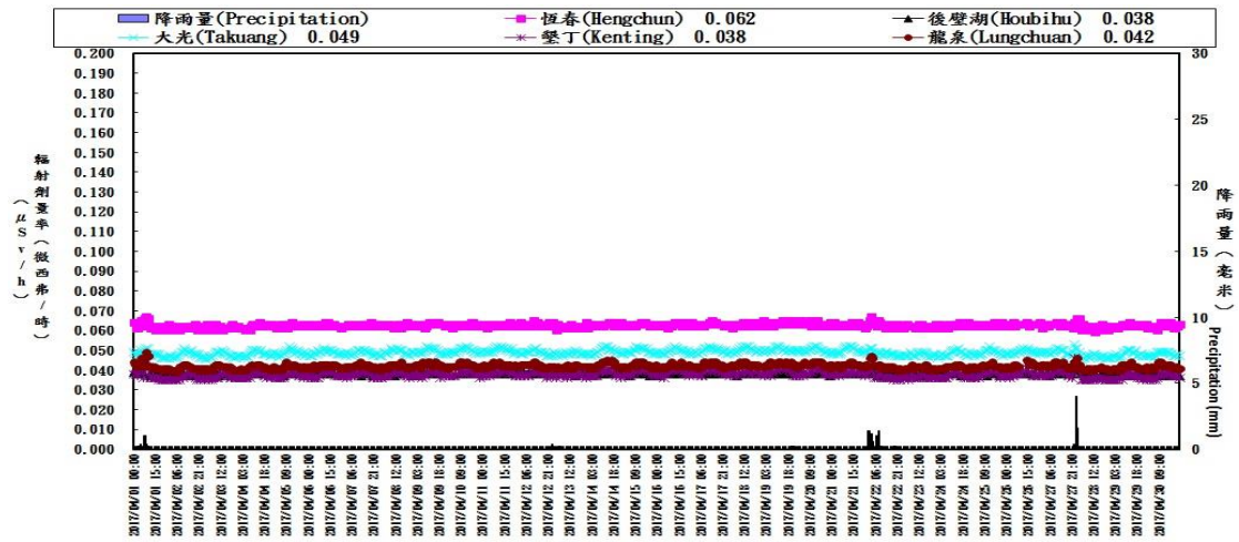
Hourly average dose rates around NPP3 in Taiwan (April, 2017)
