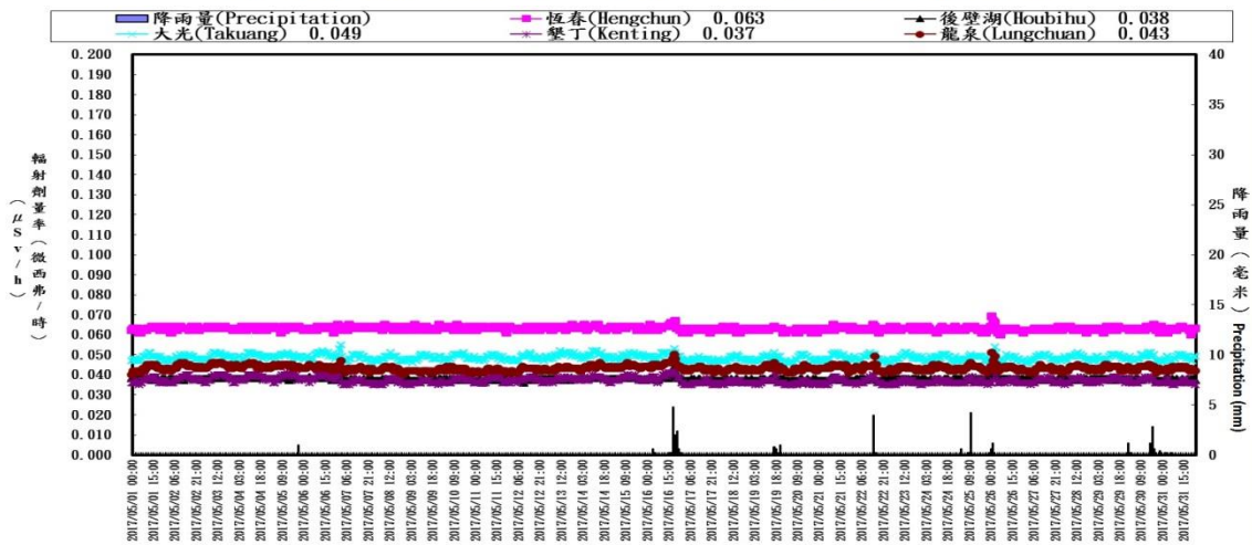
Hourly average dose rates around NPP3 in Taiwan (May, 2017)
