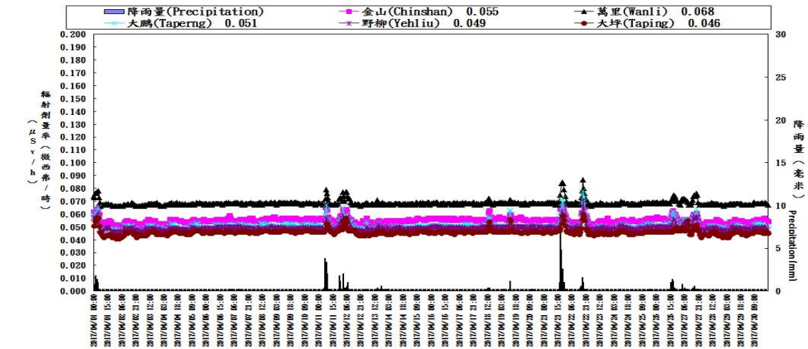
核二廠輻安預警自動監測時平均劑量率(中華民國一百零六年四月) Hourly average dose rates around NPP2 in Taiwan (April, 2017)
